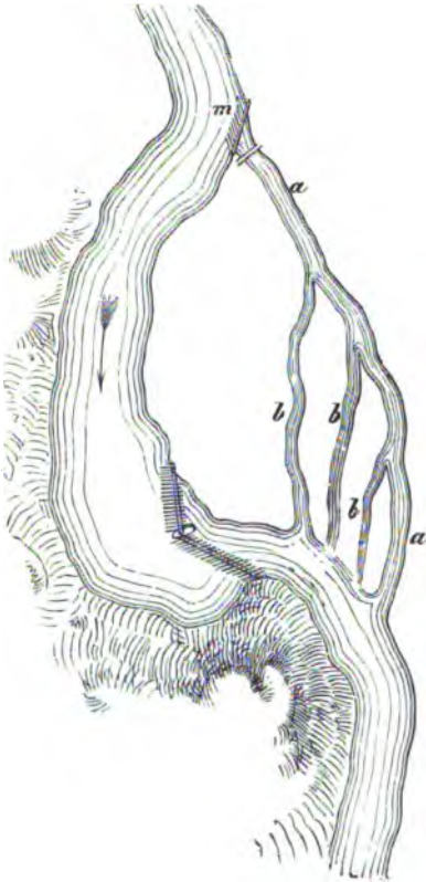
Fig. 268.—Side channel taking pressure off a boom.
